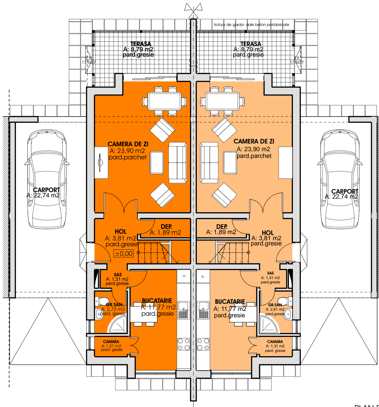
PLAN PARTER
